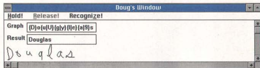
Screen 10: The symbol graph that the recognizer produces often includes alternative interpretations for characters. Dictionaries help the system arrive at a final result.
